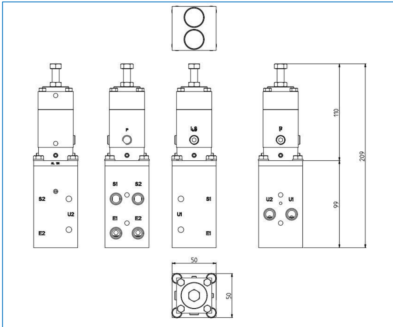
Figure 2 – Dimensional drawing
