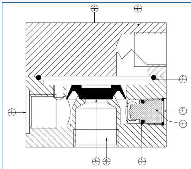
Figure 5 - Section
