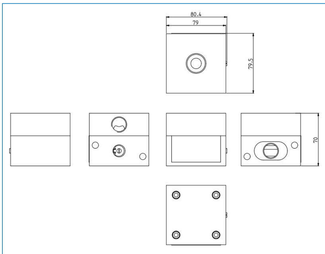
Figure 2 – Dimensional drawing
