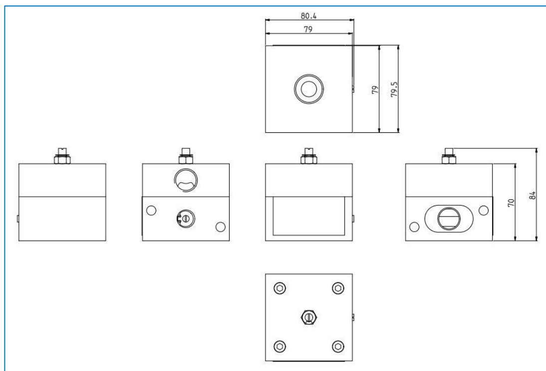
Figure 6 – Dimensional drawing
