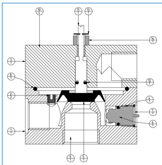
Figure 7 - Section
