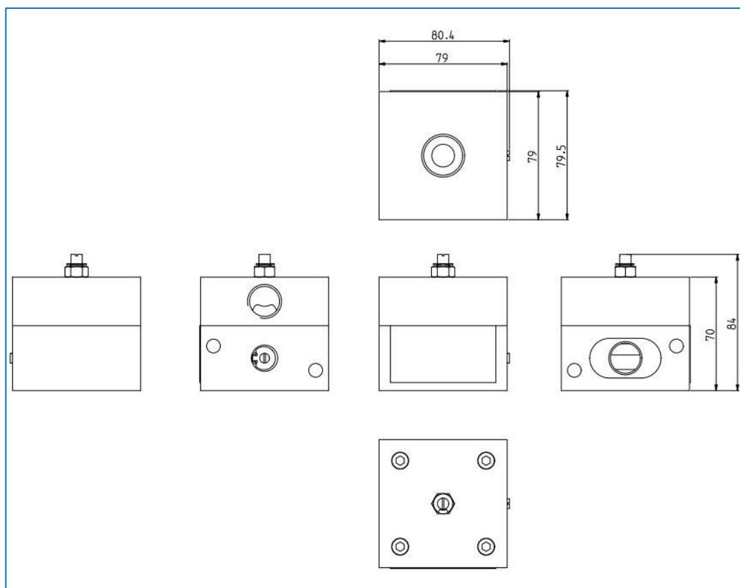
Figure 8 – Dimensional drawing
