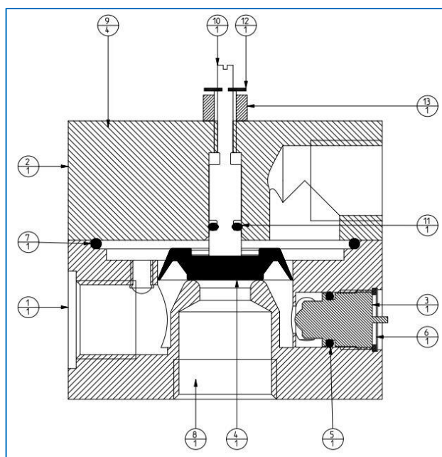
Figure 9 - Section
