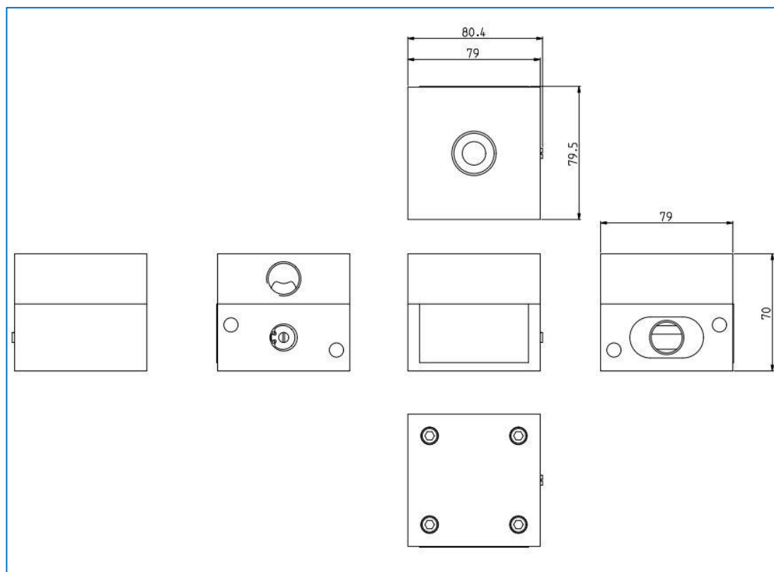
Figure 4 – Dimensional drawing
