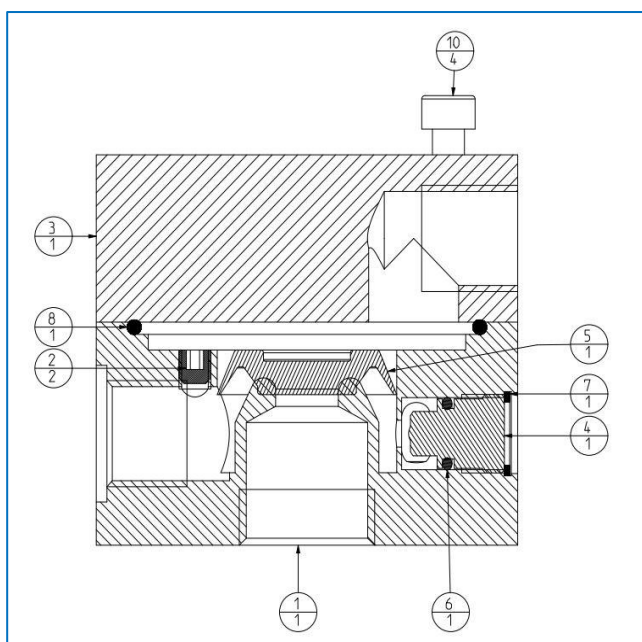
Figure 3 - Section
