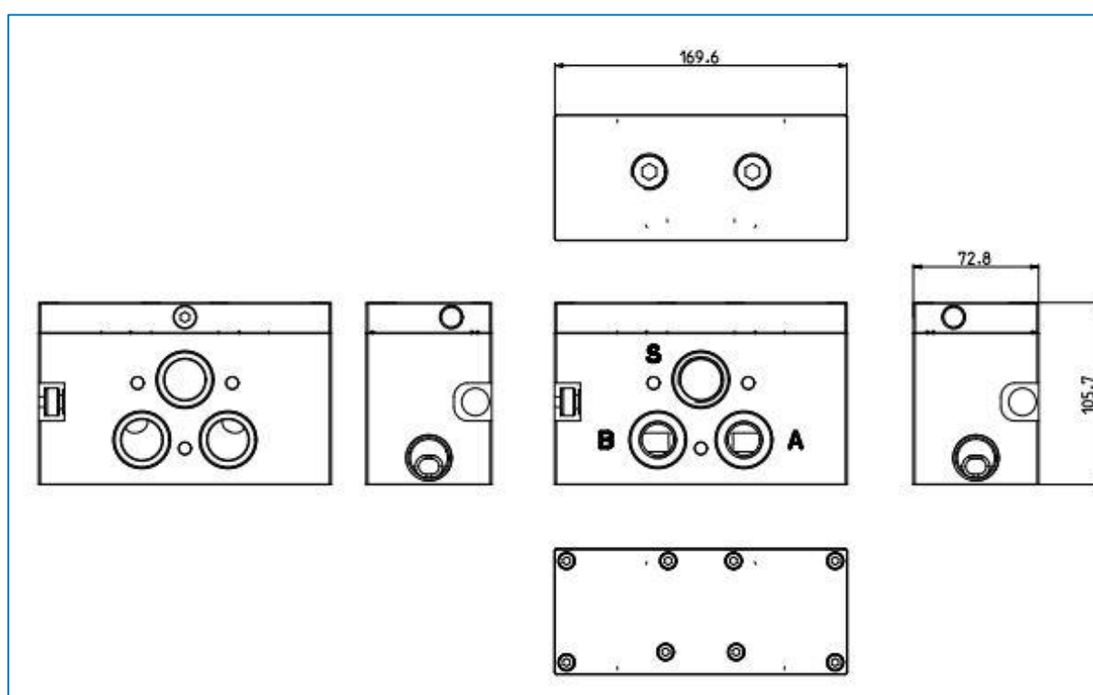
Figure 2 – Dimensional drawing
