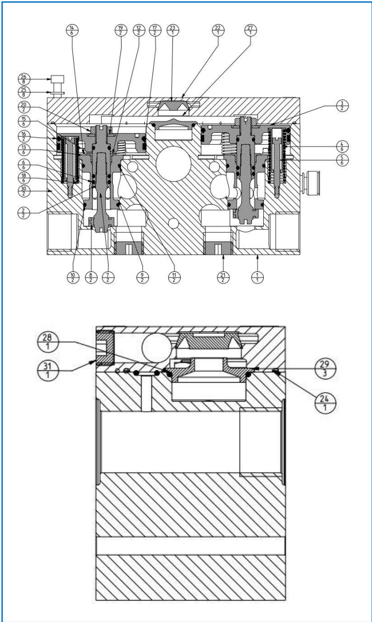
Figure 3 - Section
