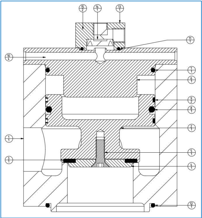
Figure 5 - Section
