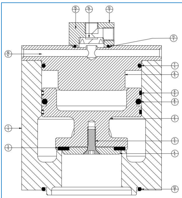
Figure 3 - Section
