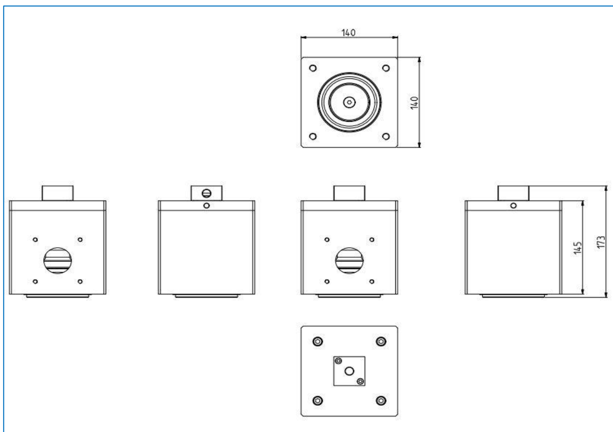
Figure 2 – Dimensional drawing
