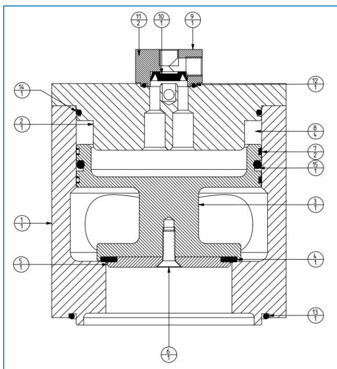
Figure 7 - Section
