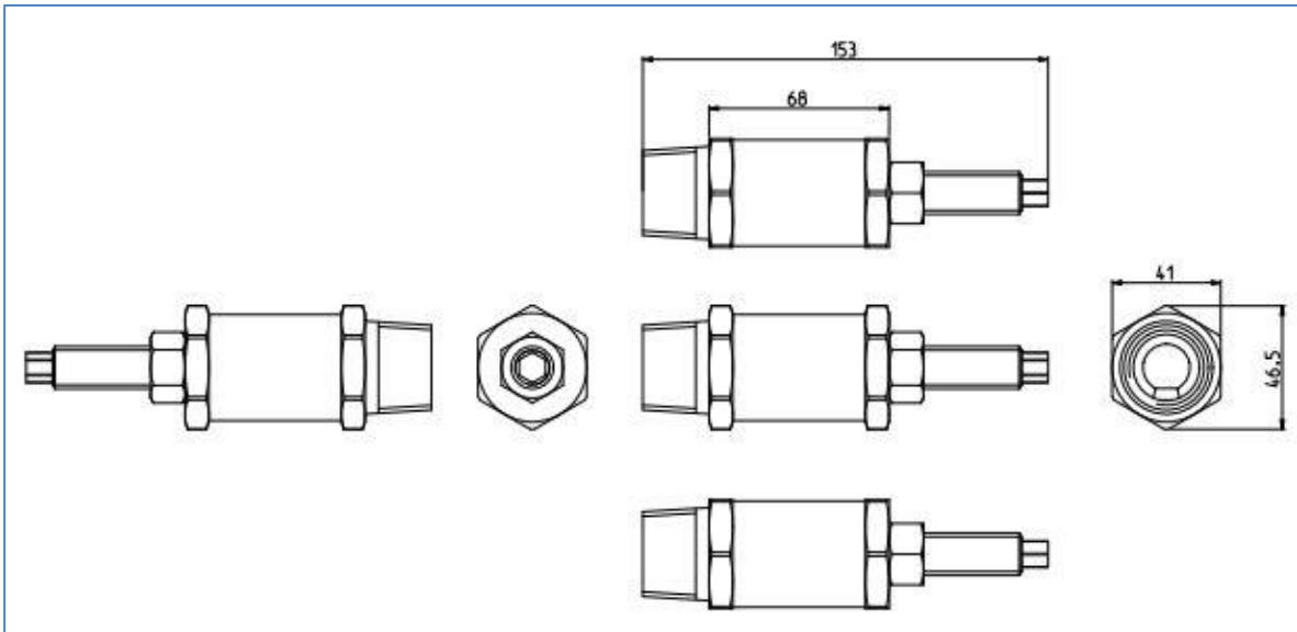
Figure 10 – Dimensional drawing
