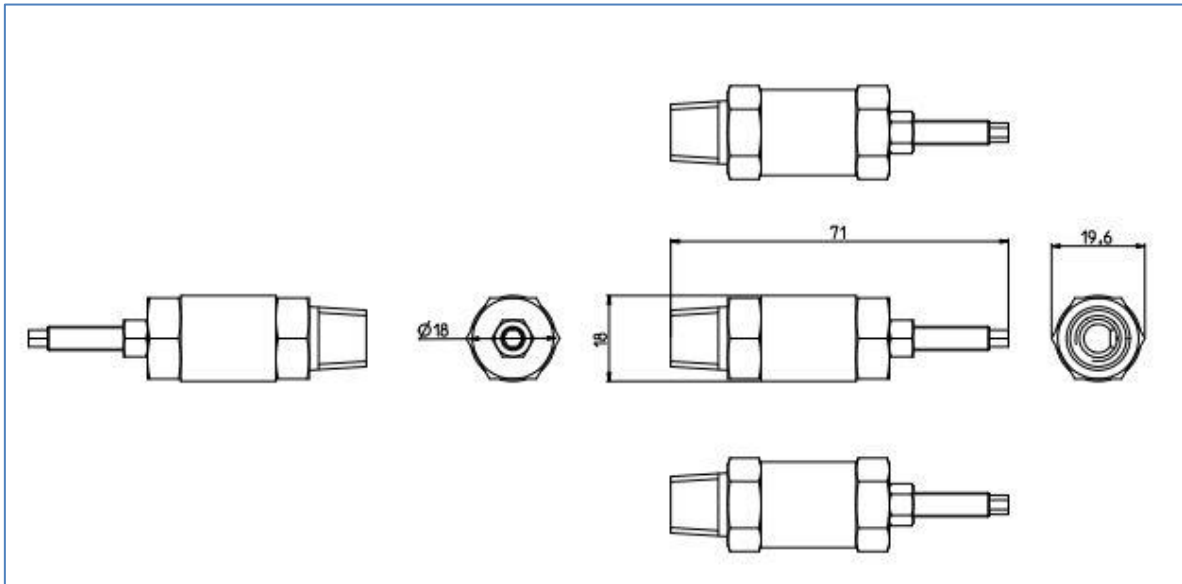
Figure 2 – Dimensional drawing
