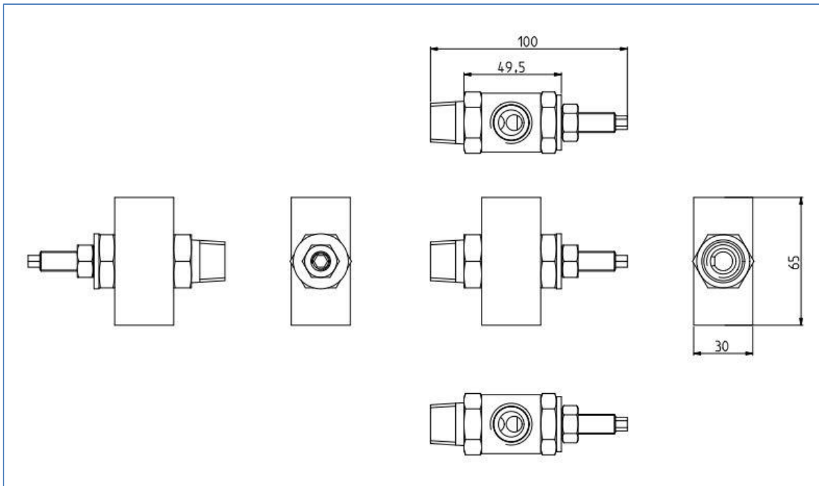
Figure 8 – Dimensional drawing
