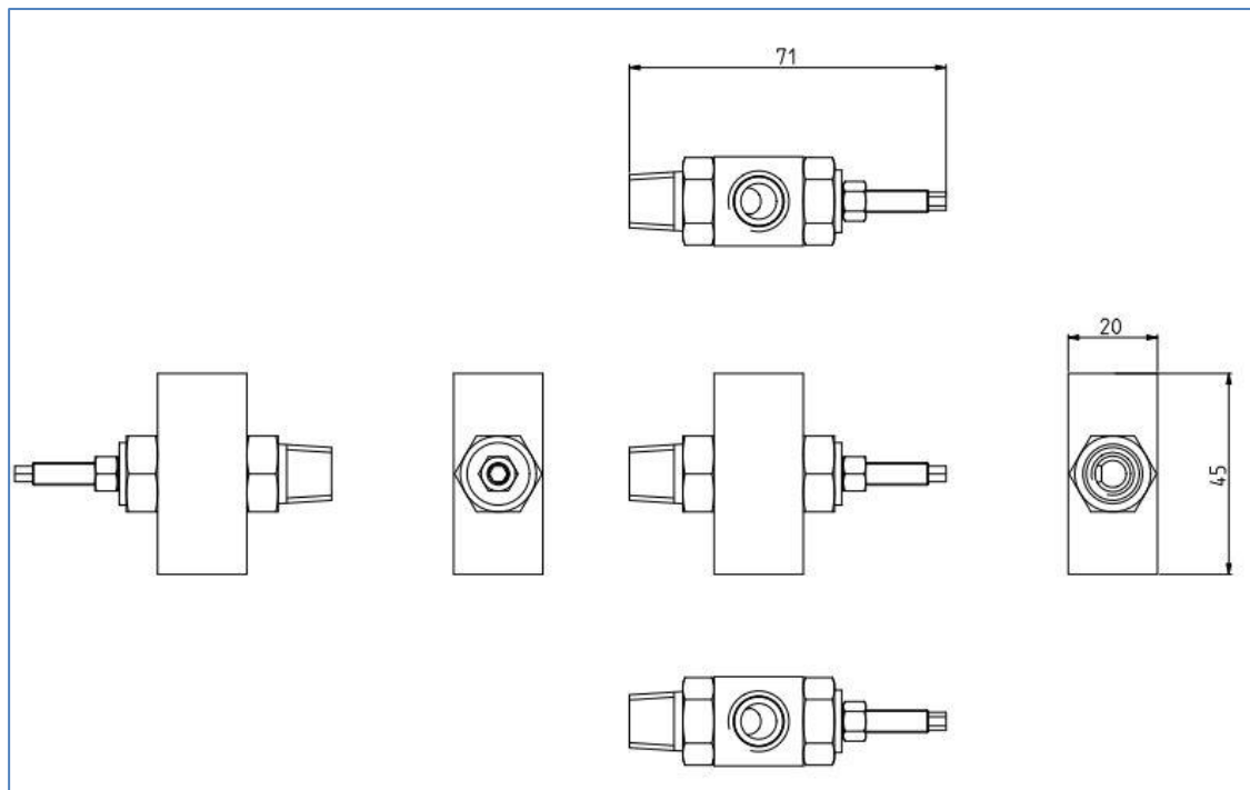
Figure 4 – Dimensional drawing
