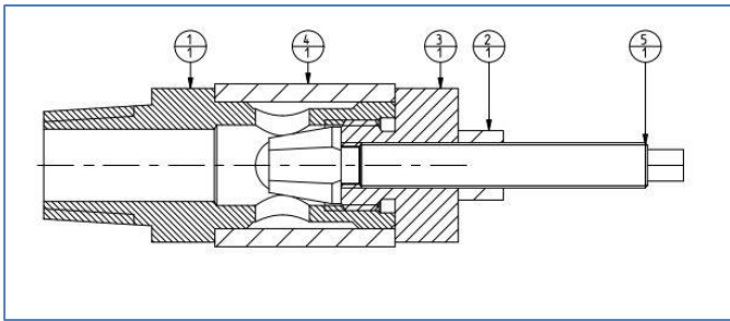
Figure 3 - Section
