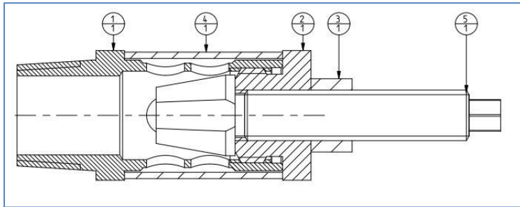
Figure 11 - Section
