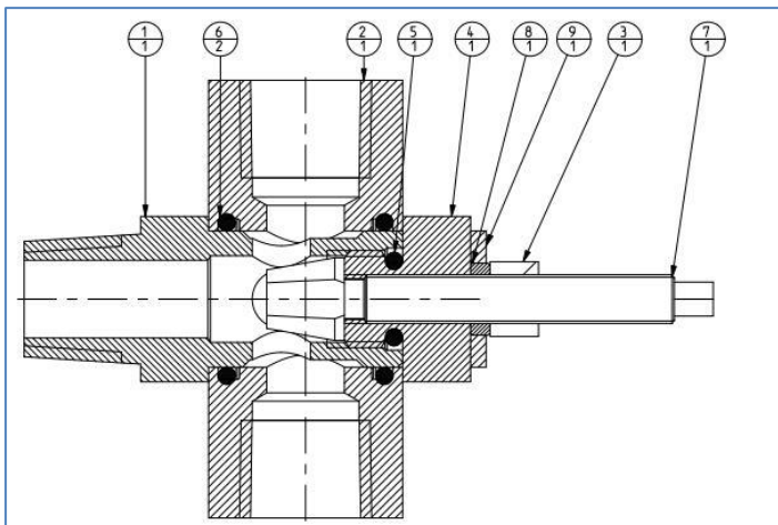
Figure 5 - Section
