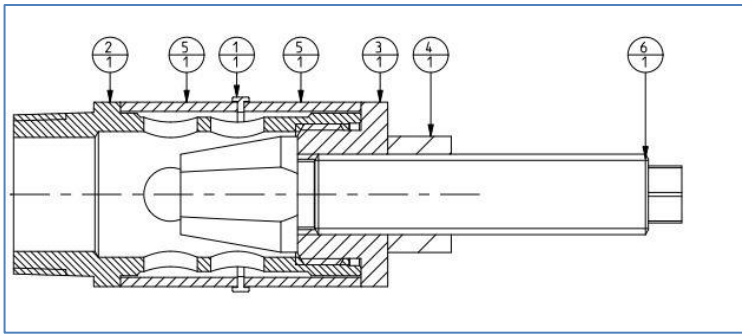
Figure 15 - Section
