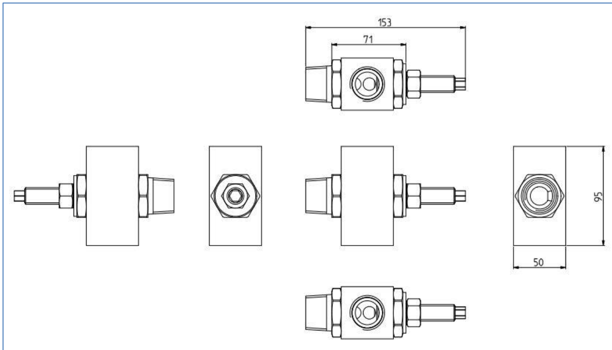
Figure 12 – Dimensional drawing
