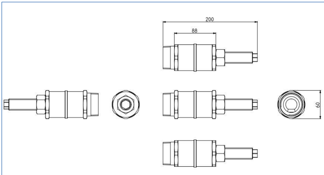
Figure 14 – Dimensional drawing
