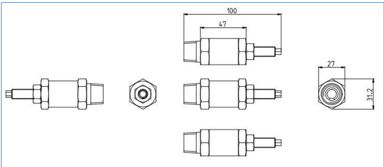
Figure 6 – Dimensional drawing
