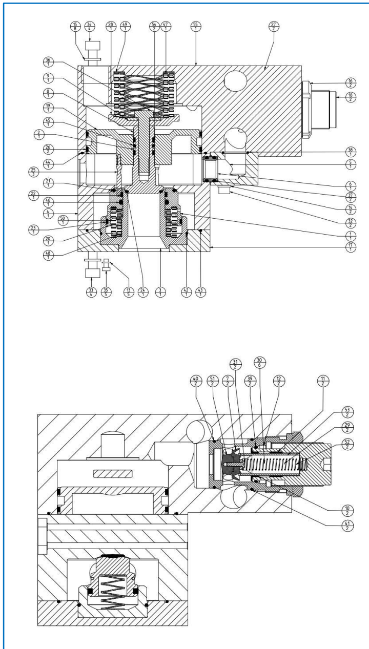
Figure 3 - Section
