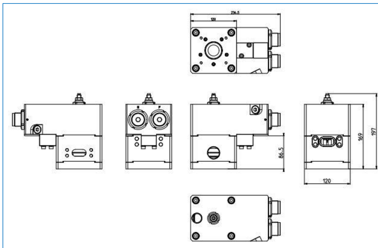
Figure 4 - Dimensional drawing
