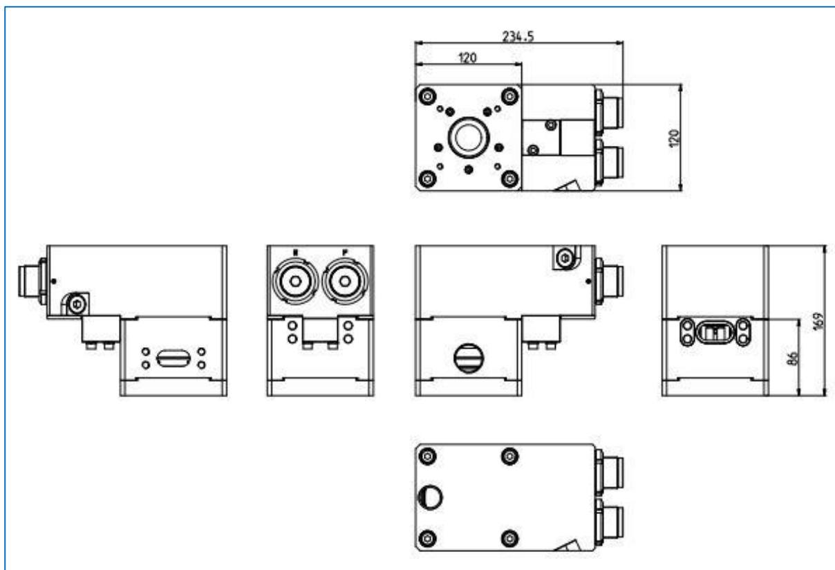
Figure 2 – Dimensional drawing
